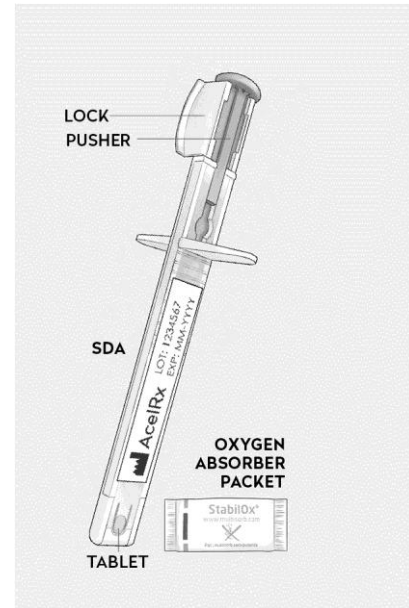
Figure 2. Lock Removal
